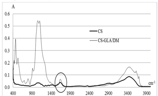
Figure 1b. The FT-IR spectra of CS and CS-GLA/DM
