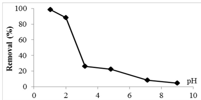
Figure 5. Effect of pH on the RO122 removal
