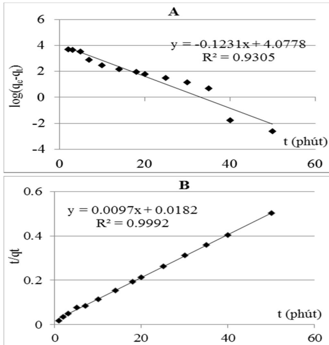
Figure 7. First-order order kinetic plot (A) and second-order kinetic plot (B) for the sorption of RO122 on CS-GLA/DM
