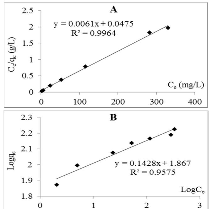
Figure 6. Adsorption isotherm linear for the adsorption of RO122 by CS-GLA/DM (A) The Langmuir isotherm and (B) The Freundlich isotherm
