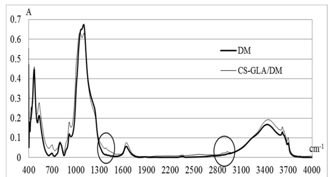
Figure 1a. The FT- IR spectra of DM and CS-GLA/DM
