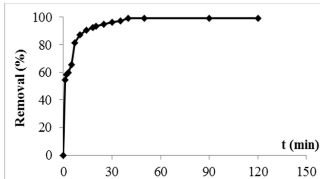
Figure 3. Effect of contact time on the RO122 removal
